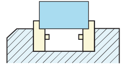
SPECIAL JAW DESIGNED FOR THIN WORKPIECE
